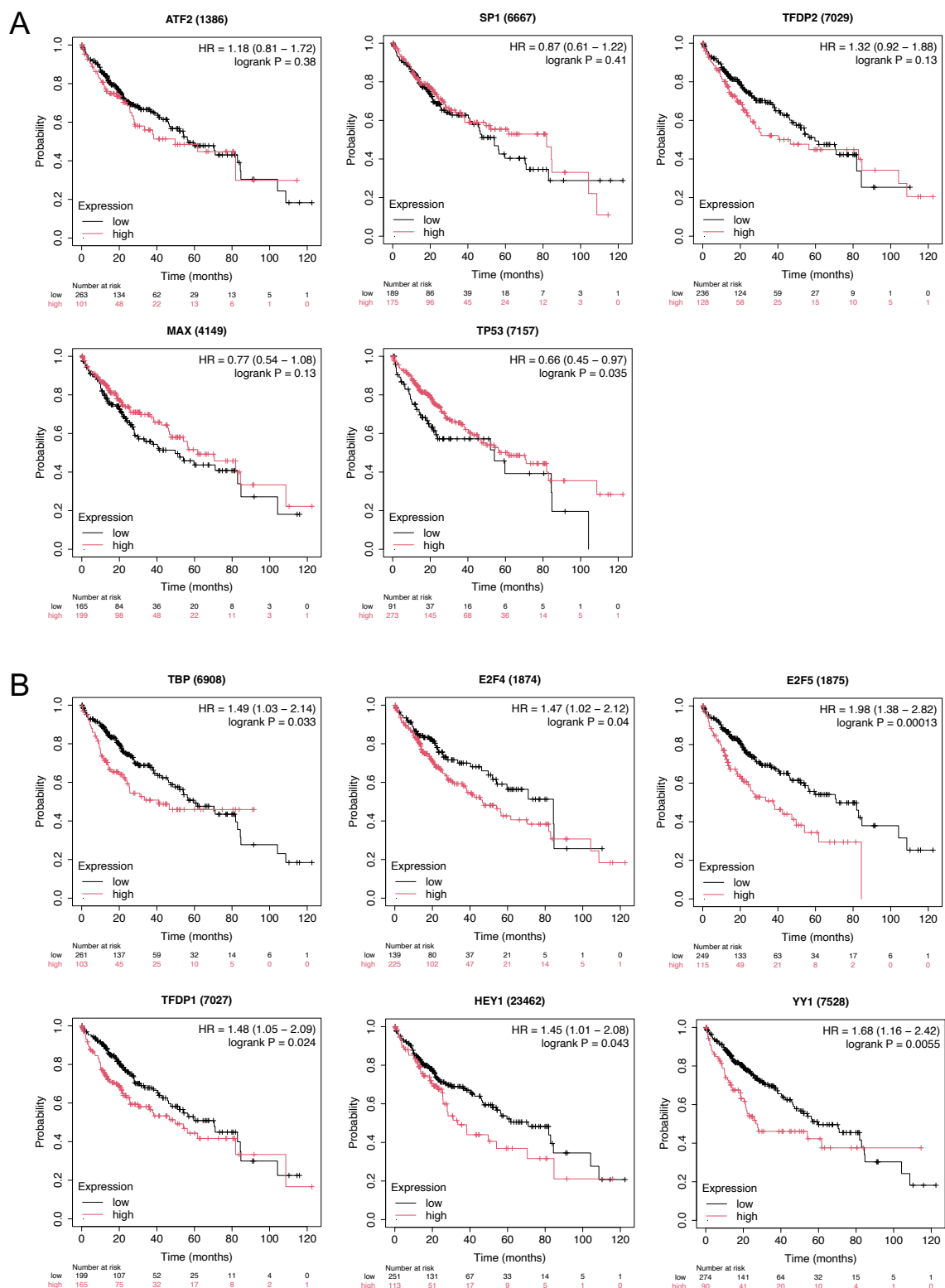
Supplemental Figure S5. KM Plotter ( https://kmplot.com/ ) output. (A) Graphs from KM Plotter for liver cancer show time in months (x-axis) plotted against the survival probability (y-axis) for non-reproducible cases. Legends at the top and bottom show Hazard ratio (HR) for relative risks (death, relapse) and logrank p-values and indicate the color code for high (red) and low (black) expression, respectively. Risk numbers are indicated for high/low expression at each time point at the bottom. (B) Graphs from KM Plotter show time in months (x-axis) plotted against the survival probability (y-axis) for reproducible cases like in panel A.
