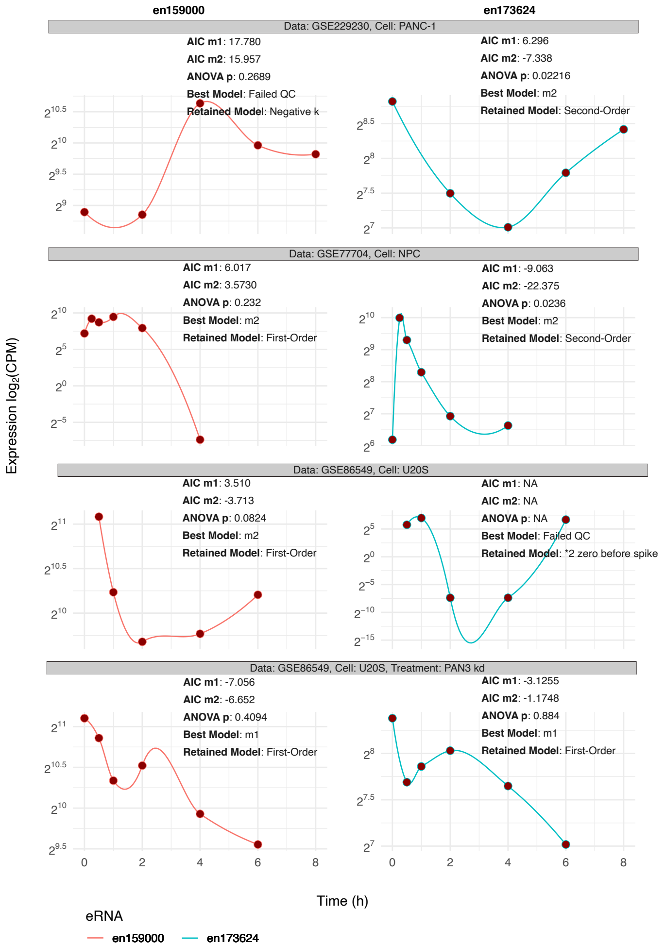
Figure S3. Example eRNA decay curves illustrating fitting of first-order exponential decay and second-order kinetic models to CPM-normalized eRNA time-course data. Cases where second-order models provide a better fit, and quality control issues such as negative decay rates or transient spikes following consecutive zero-expression measurements are annotated.
