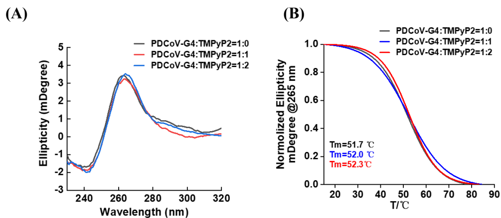
Figure S2. TMPyP2 did not affect the topological conformation or the thermal stability of PDCoV-G4. (A) CD spectra analysis of PDCoV-G4 in the presence of different concentrations of TMPyP2. (B) The normalized data from the CD thermal melting curves of PDCoV-G4 in the presence of different concentrations of TMPyP2.
