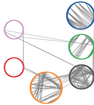
S5 Fig. Network visualizations of SIG5 protein isoforms undergoing an isoform switch. Protein structure network representations of (a) SIG5_P1 and (b) SIG5_c2. Circles represent clusters that correspond to Infomap communities (see methods).
