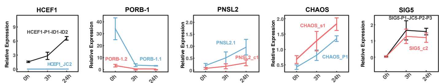
S2 Fig. Validation of RNA-Seq profiles of photosynthesis related genes by qPCR. Each plot contains transcripts of a gene identified as undergoing isoform switch. Errors bars represent SD values. Names of the respective transcripts are shown in the same color of the profile that they represent. Black profiles represent cases where primers did not distinguish some transcripts, indicating the expression of more than one transcript. All associated transcripts are represented by the respective black profile.
