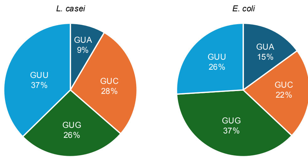
Fig. S6. Proportion of valine codon (GUA, GUC, GUG, and GUU) usage in L. casei (left) and E. coli (right).
