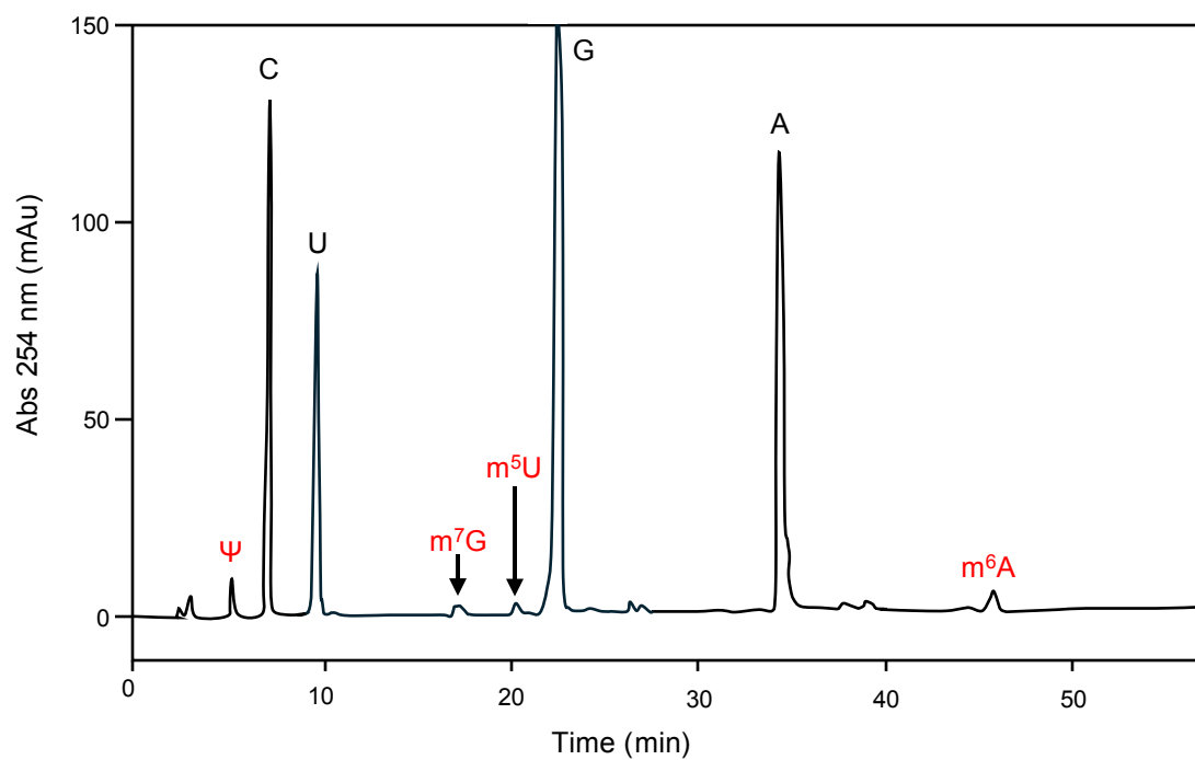
Fig. S5. Nucleoside analysis of tRNA Val from L. casei . Peaks with the elution time corresponding to those for Ψ, m 7 G, m 5 U, and m 6 A were detected.
