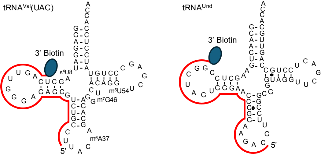
Fig. S3. DNA probes for isolation of tRNA Val and tRNA Und . The positions of the 3'-biotin DNA probe for tRNA isolation are indicated by red lines.
