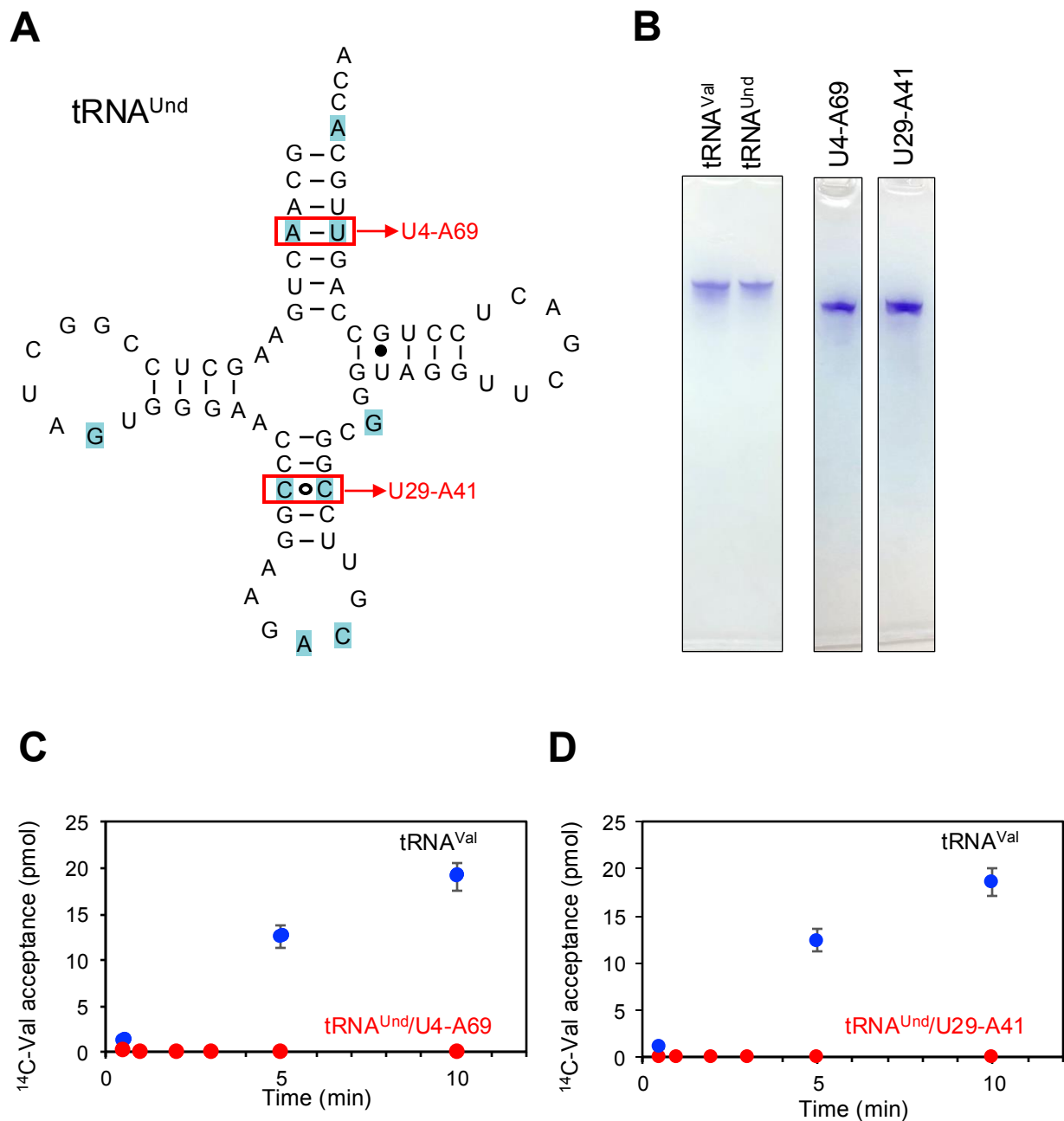
Fig. S1. Val acceptance activity of tRNA Und mutant transcripts by ValRS. (A) The tRNA determinants of E. coli ValRS are highlighted in cyan. (B) In vitro transcribed tRNAs were analyzed by 10% PAGE (7 M urea). The gels were stained with toluidine blue. (C) Val acceptance activities of tRNA Und transcripts with A4-U-69 substituted for U4-A69 or (D) C29•C41 substituted for U29-A41. Blue and red circles represent tRNA Val and tRNA Und mutants, respectively.
