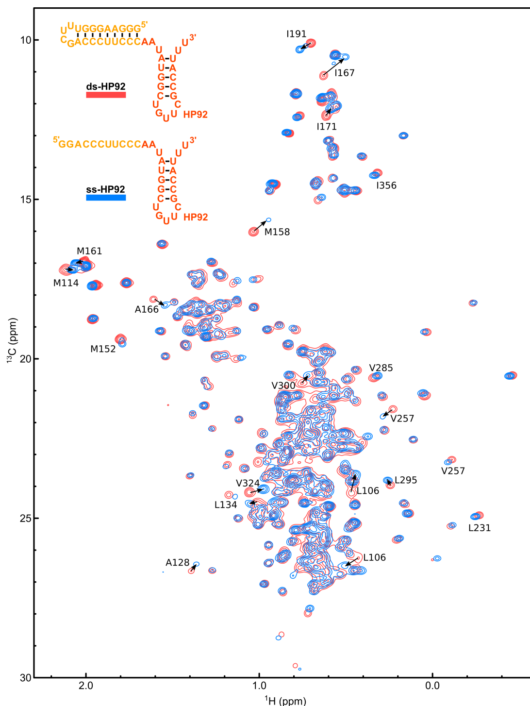
Supplementary Fig. 6: Spectra of DbpA/ADP/BeF 3 in complex with and ss-HP92 and hp-HP92 complex are similar, but display marked differences.
