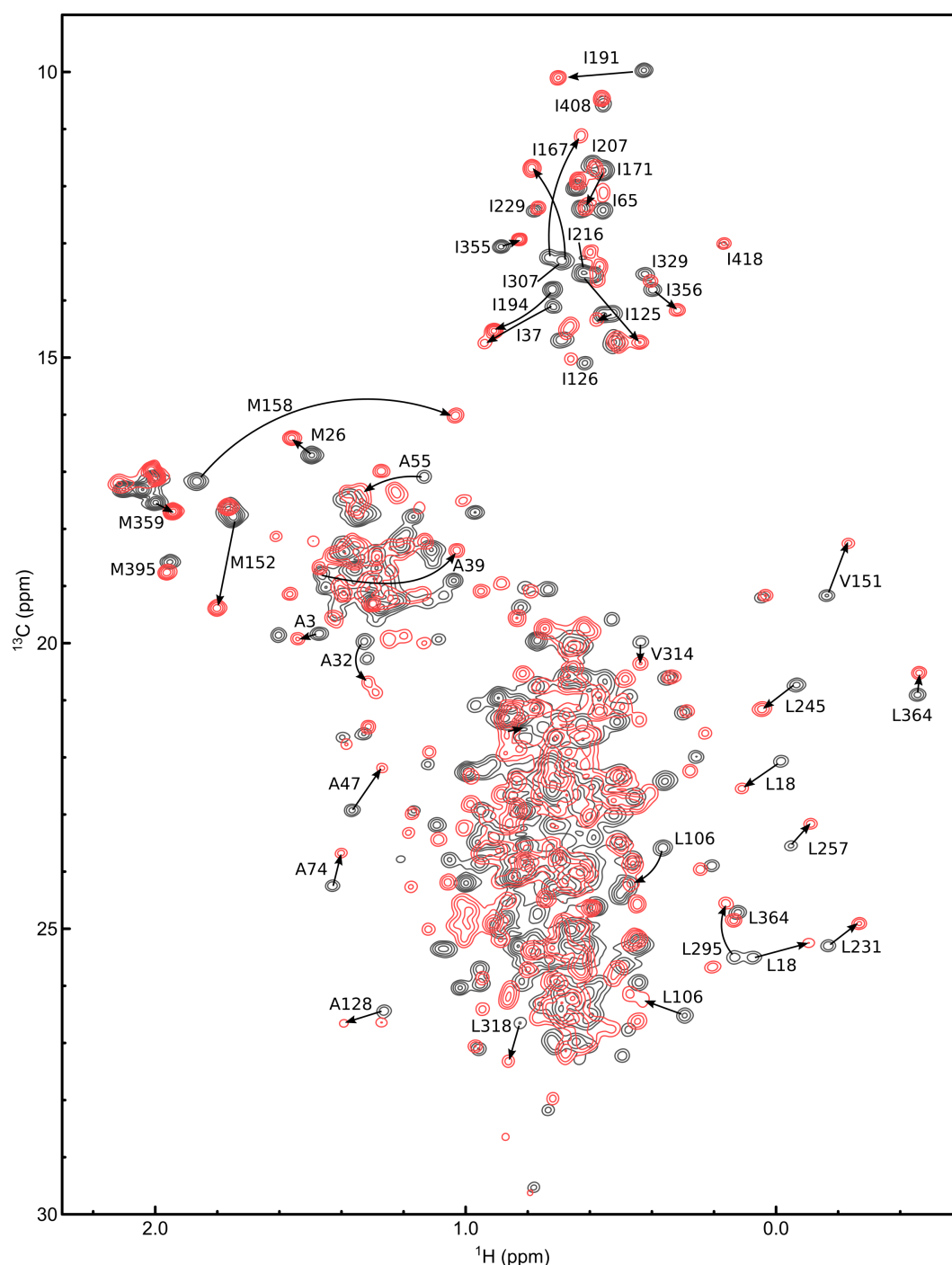
Supplementary Fig. 5: Binding of ADP/BeF 3 to the hp-HP92/DbpA complex followed by methyl NMR.
