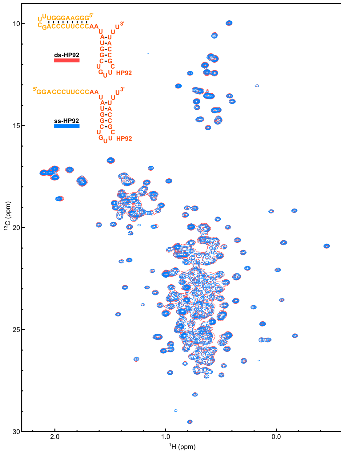
Supplementary Fig. 4: Spectra of DbpA in complex with ss-HP92 and hp-HP92 RNAs are virtually identical.
