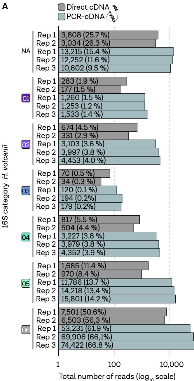
Fig. S9 | Relative and absolute quantification of rRNA intermediates in H. volcanii .
