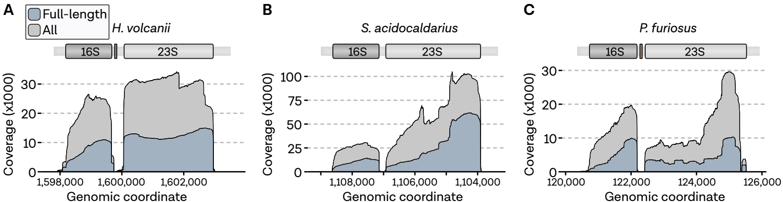
Fig. S4 | Coverage profile comparison of full-length and unfiltered reads.
