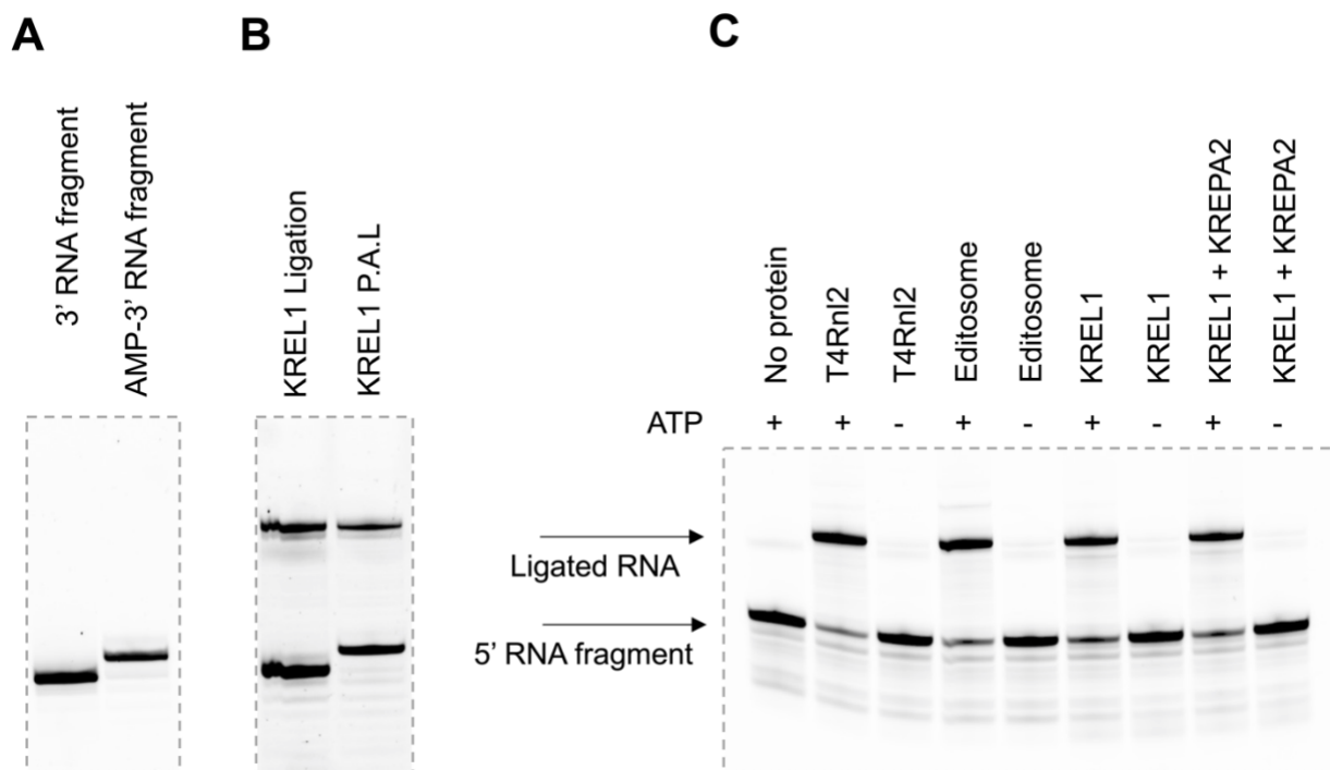
Supplemental Figure S6. Control experiments for ligation assays. (A) 3' RNA fragment migrated alongside the adenylylated 3' RNA fragment in a 20% acrylamide gel. (B) Ligation of unadenylylated RNA with ATP alongside ligation of pre-adenylylated RNA in the absence of ATP. (C) Three-step ligation assay of T4 RNA ligase 2 (T4Rnl2), the whole editosome, and KREL1 with and without KREPA2, in the presence and absence of ATP.
