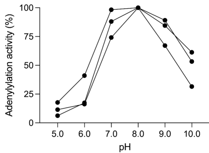
Supplemental Figure S5. KREL1 adenylylation activity in pH 5-10. Reactions include 25 mM Tris-HCl of pH 5-8 or 25-mM Tris-Acetate pH 9-10.
