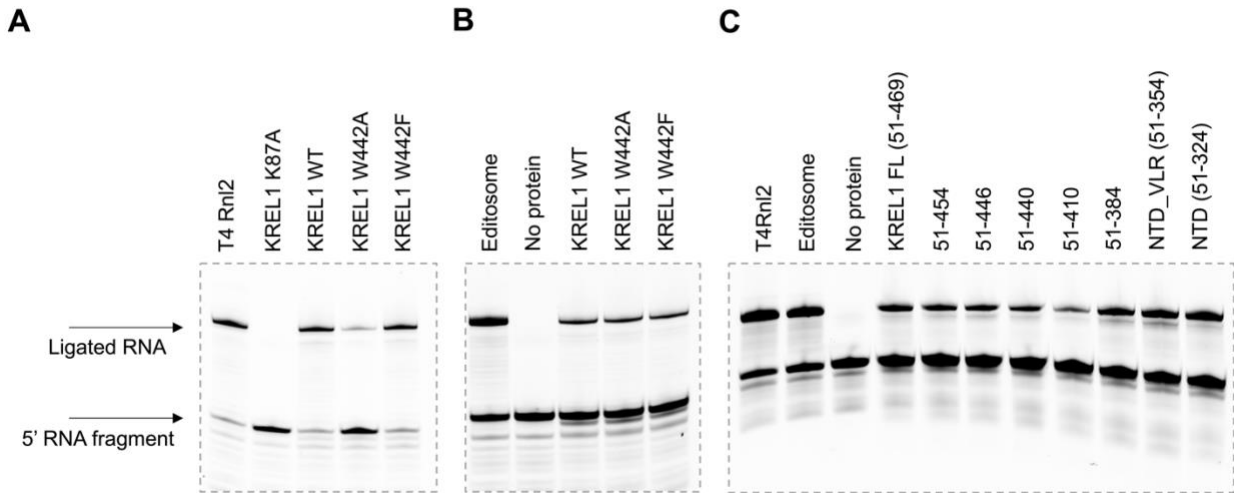
Supplemental Figure S4. The activity of motif VI mutants in ligation and pre-adenylylated ligation assays. (A) Three-step ligation assay of T4Rnl2, KREL1 WT and W442 mutants. Point mutation K87A is a negative control. (B) Pre-adenylylated ligation assay of the editosome, KREL1 WT and W442 mutants. (C) Pre-adenylylated ligation assay of the KREL1 FL (51-469) and CTD truncations.
