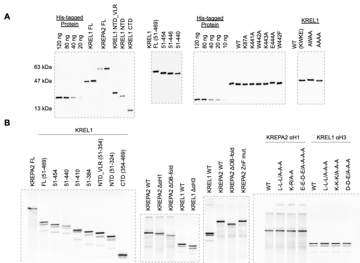
Supplemental Figure S2. Expression of KREL1 and KREPA2 recombinant proteins. (A) Western blots using an anti-his-tagged antibody against KREL1 FL, independent domains, CTD truncations, point mutants, and group mutants. (B) SDS-PAGE gels showing expression of the radiolabeled recombinant proteins expressed with S35 methionine and visualized using the PhosphorImager.
