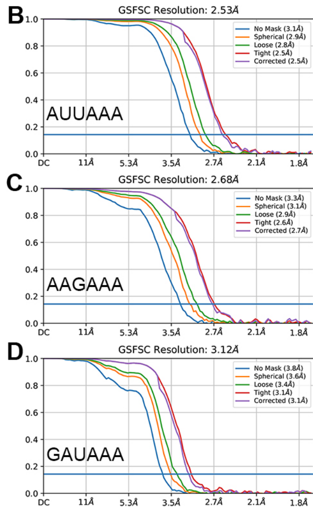
Fig. S1. (A). A flowchart showing the general protocols for EM data processing and image reconstruction. (B). FSC curves for the AUUAAA reconstruction. (C). FSC curves for the AAGAAA reconstruction. (D). FSC curves for the GAUAAA reconstruction.
