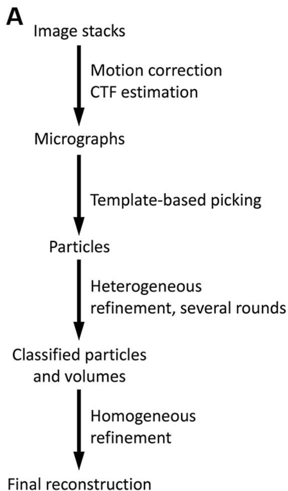
Fig. S1. (A). A flowchart showing the general protocols for EM data processing and image reconstruction. (B). FSC curves for the AUUAAA reconstruction. (C). FSC curves for the AAGAAA reconstruction. (D). FSC curves for the GAUAAA reconstruction.
