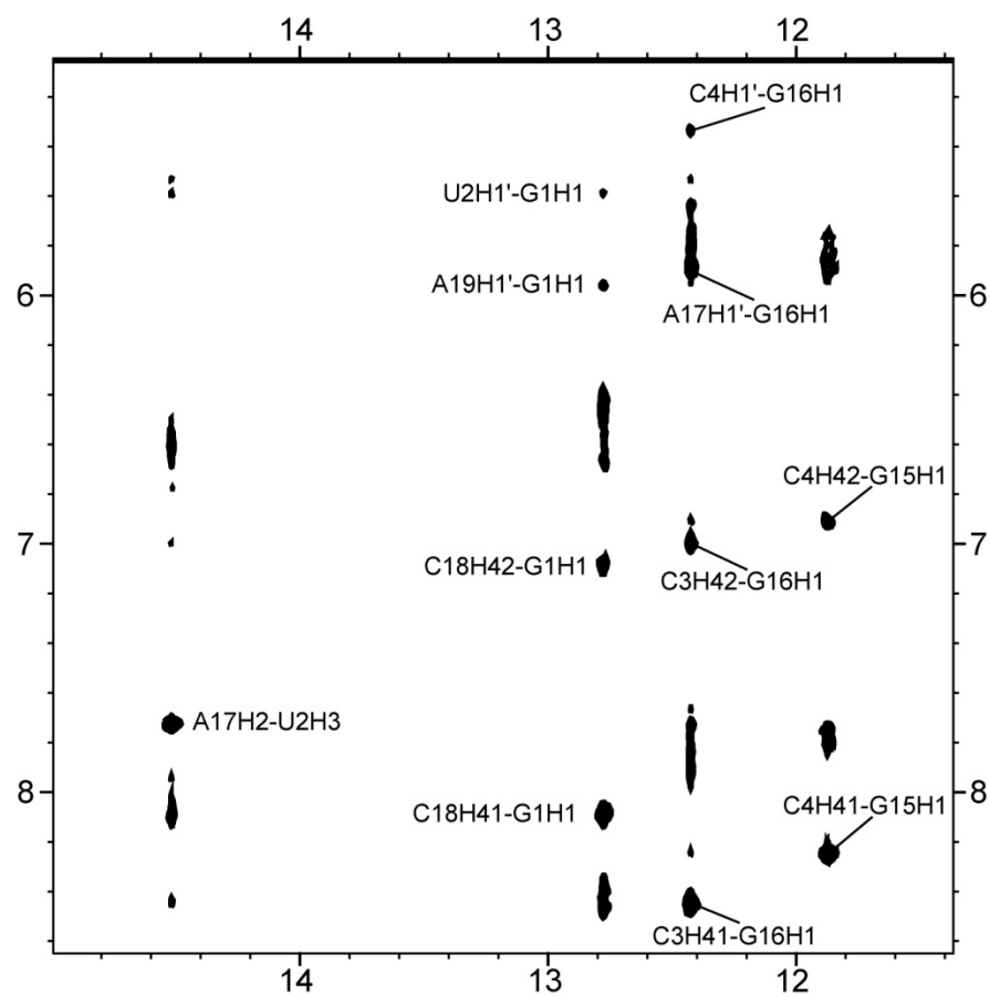
Supplemental Figure S2) 2D Watergate-NOESY spectrum of HP1 at 0 °C and mix time 150 msec. Cross-peaks typical of the expected secondary structure are indicated.
