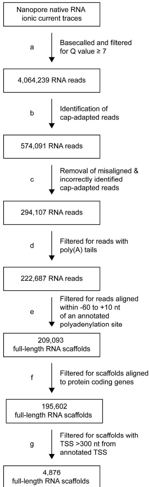
Supplementary Figure 7 Nanopore data processing steps. Each arrow represents a computational step. Each box represents the type and quantity of data after a computational step.
