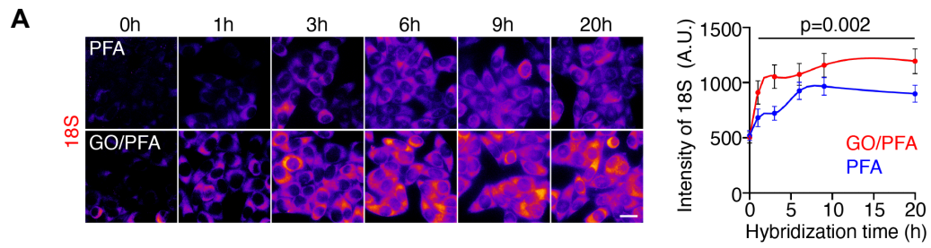
Figure S2. Glyoxal/PFA fixation improves RNA FISH efficiency by enhancing probe accessibility
