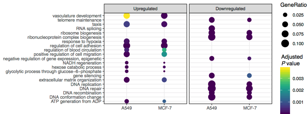
Supplementary Figure 2. Gene ontology (GO) analyses of the differentially expressed genes under hypoxia. GeneRatio refers to the fraction of the tested genes that is associated with the given category. A GeneRatio of 0.025 signifies that 2.5% of the tested genes are associated with the respective term.
