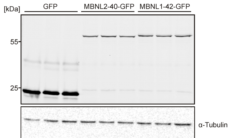
Supplementary Figure 17. MBNL1-42 and MBNL2-40 have equal overexpression efficiencies. Fluorescence detection of GFP, MBNL1-42-GFP and MBNL2-40-GFP shows equal MBNL1-42-GFP and MBNL2-40-GFP levels. Western blot analysis of \alpha -Tubulin was performed as loading control. n = 3.
