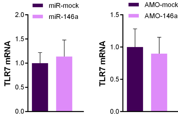
Figure S1. TLR7 mRNA expression in the cells with miR-146a or AMO-146a. HeLa cells were transfected with miR-146a mimics or AMO-146a, and infected with CVB3 (MOI = 1) 24 h post-transfection. TLR7 mRNA abundance was quantified by RT-qPCR with \Delta\Delta C_T method. The mRNA abundance of TLR7 was normalized by GAPDH mRNA. Error bars represent SD, n = 4 .
