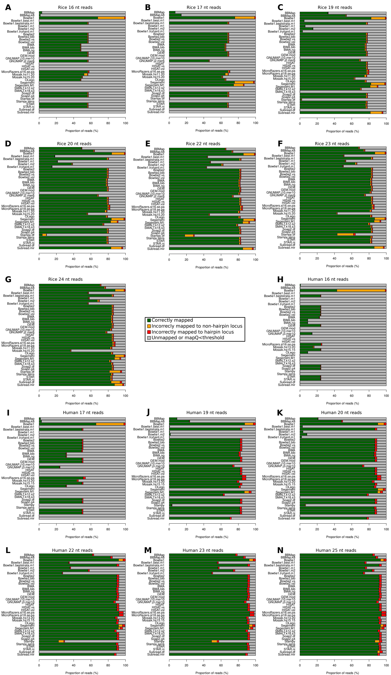
Supplementary Figure 1. Alignment of perfectly matching hairpin-derived sequence reads of varying length.
