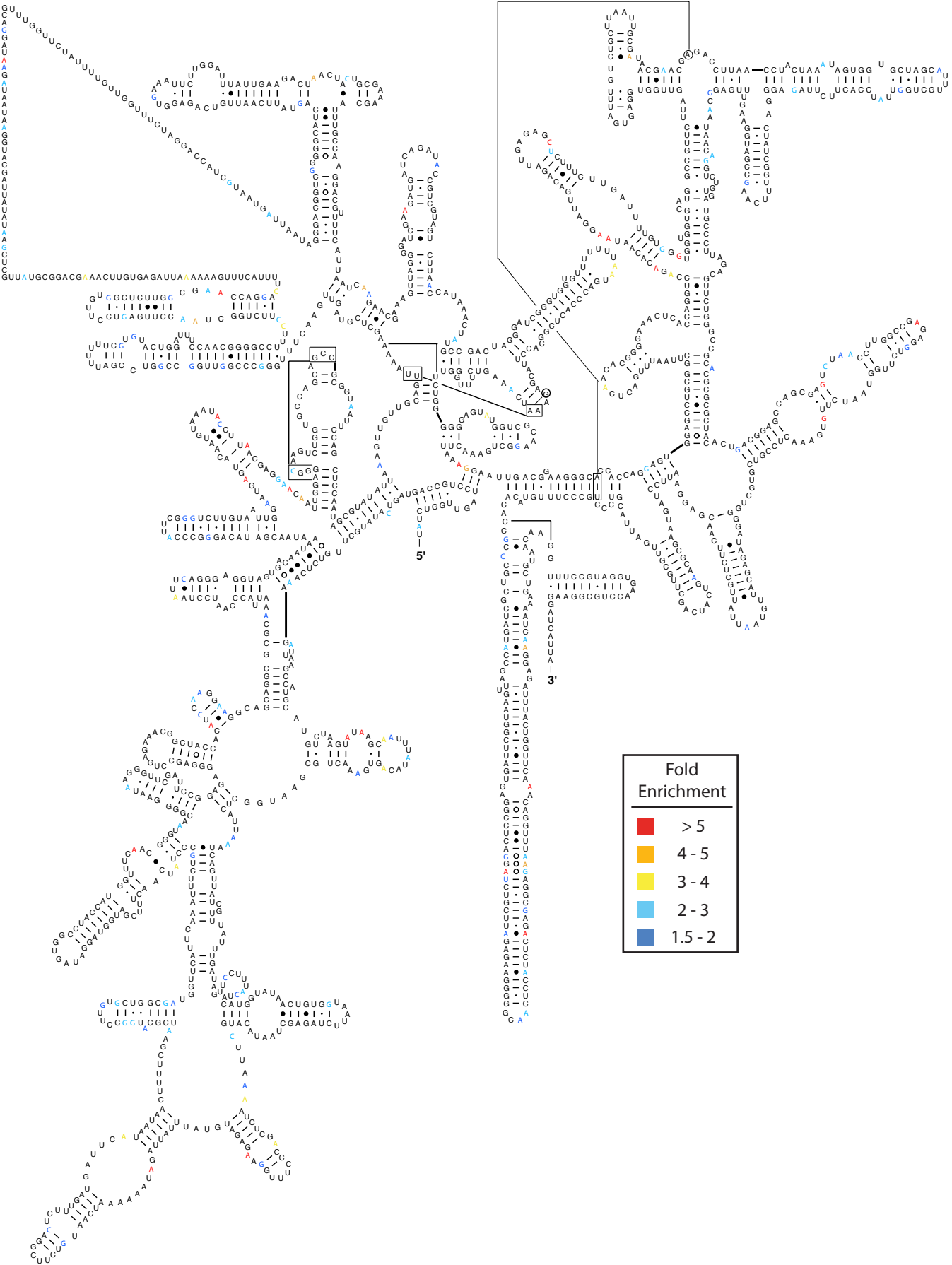
Figure S3-C Secondary structure model of the 18S rRNA.
