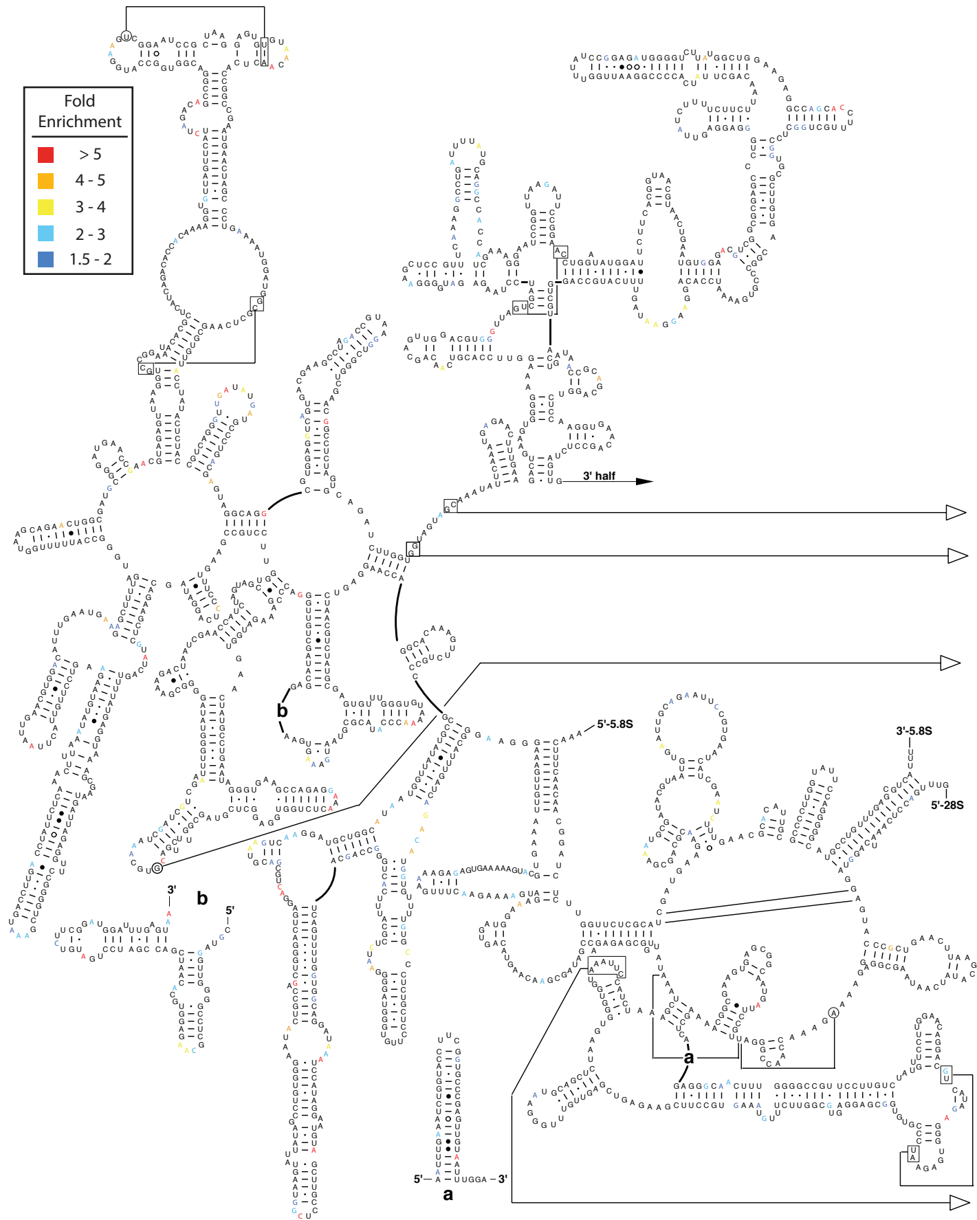
Figure S3-A. Secondary structure model of 5.8S and the 5' end of 25S rRNAs.
