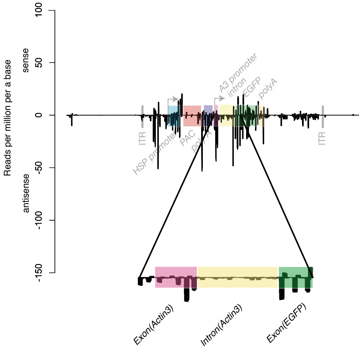
Fig. S3. Merged picture of transgene-derived piRNAs in #3 and the vector map, related to Fig. 4
